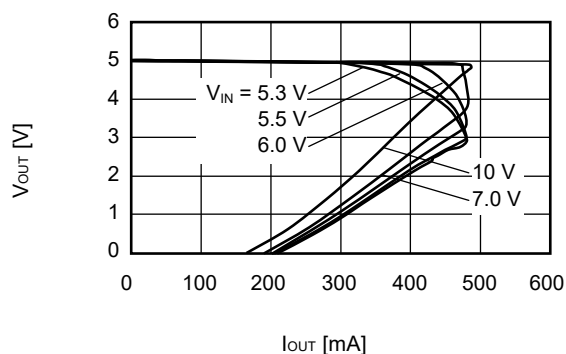
S-1200B50 ( T_a=+25^\circ\text{C} )
