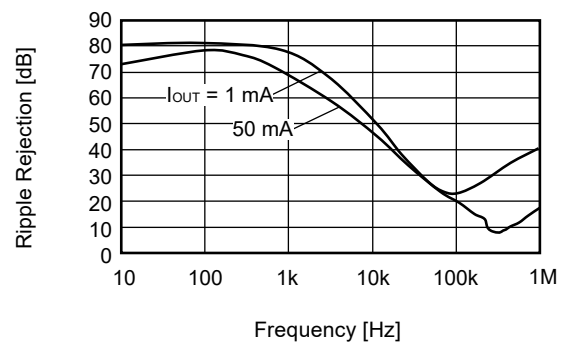
S-1200B30 ( T_a = +25^{\circ}\text{C} )
