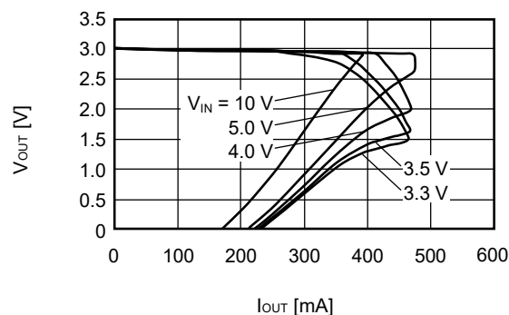
S-1200B30 ( T_a=+25^\circ\text{C} )
