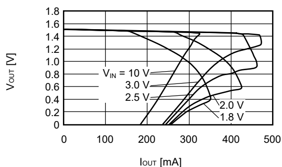
S-1200B50 ( T_a=+25^\circ\text{C} )
