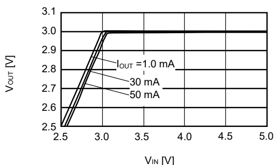
S-1200B30 ( T_a=+25^\circ\text{C} )
